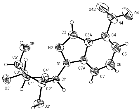
Figure 1. Perspective view of compound 1b .
