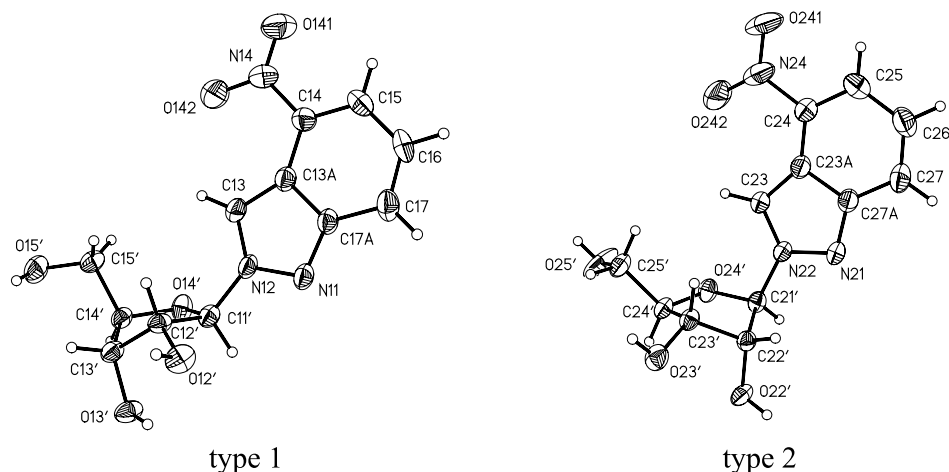
Figure 2. Perspective view of compound 2b . Type 1: S -conformation; type 2: N -conformation.
