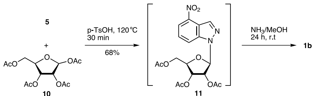
Scheme 3. The synthesis of 4-nitroindazole N 1 -( \beta -D-ribose nucleosides) by fusion reaction.
