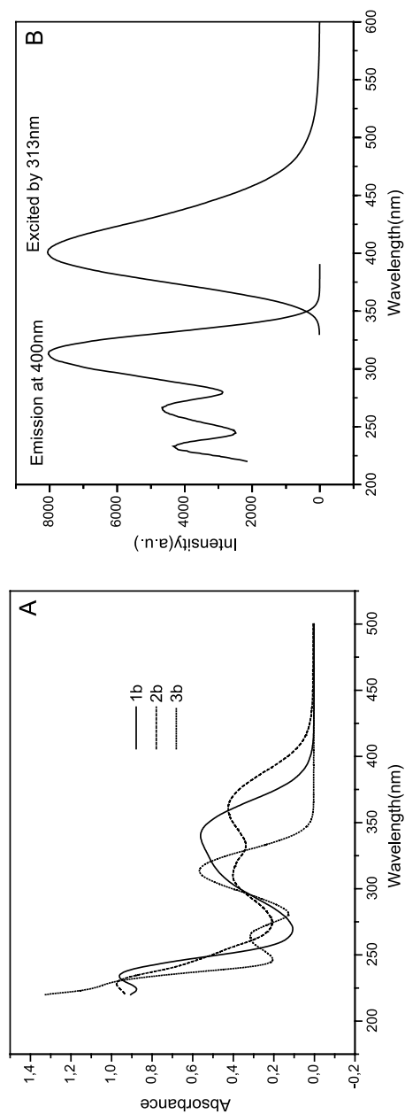
Figure 3. A: The absorption spectra of compounds 1b , 2b , 3b at room temperature. B: The emission and excitation spectra of 3b at room temperature. Solvent: methanol; concentration: C_{1b} = 8.25 \times 10^{-5} M, C_{2b} = 6.64 \times 10^{-5} M, C_{3b} = 6.83 \times 10^{-5} M.
