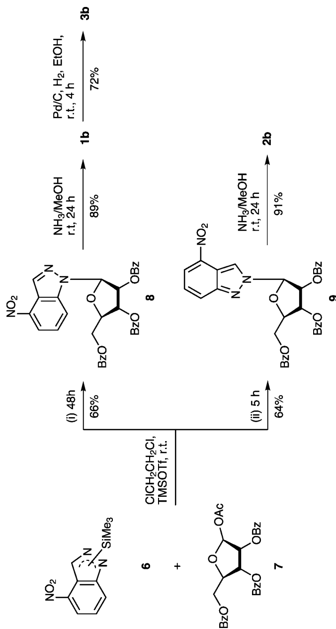
Scheme 2. The Silyl-Hilbert-Johnson glycosylation.
